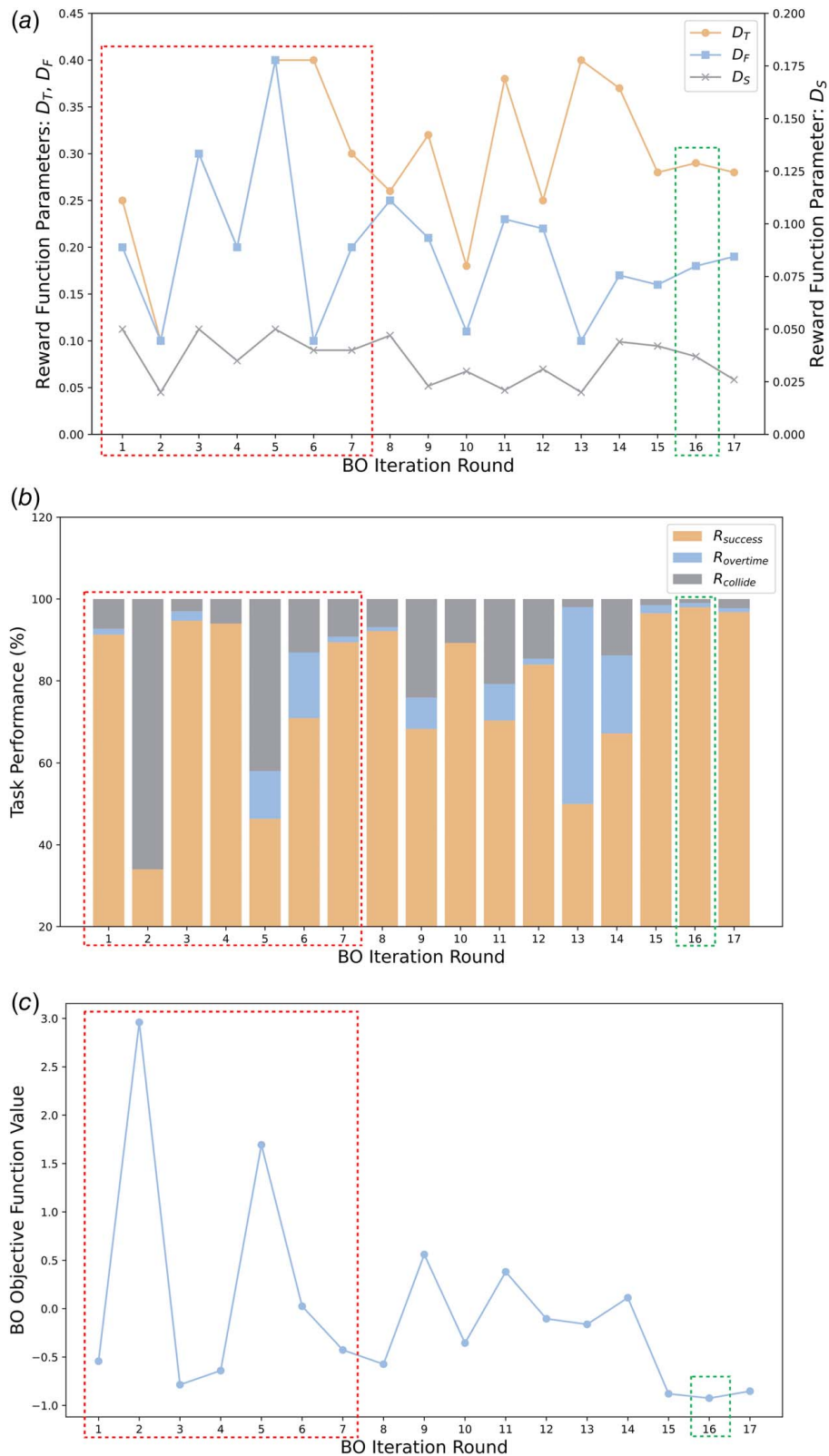
Fig. 8 Bayesian Optimization iteration results: (a) Reward function parameters of each iteration, (b) task performance of each iteration. Here, the results are the average values over five tasks. (c) Objective function value of each iteration. The dashed boxes on the left highlight the first seven iterations trained with initially selected parameters. The dashed boxes on the right show the 16th iteration with the best performance.
