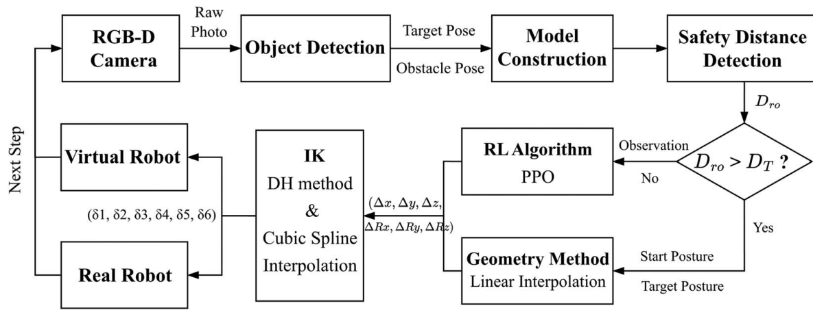
Fig. 3 The workflow of adaptive motion planning method
