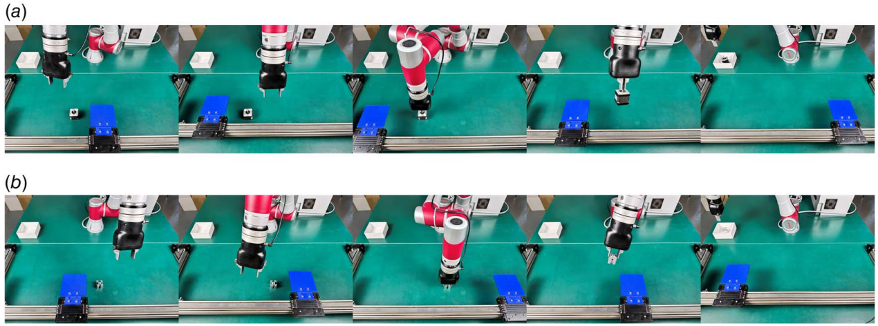
Fig. 16 Physical scenes of Pick and Place tasks for stepping motor and aluminum profile. The figure from left to right shows the obstacle avoidance process of the proposed method.
