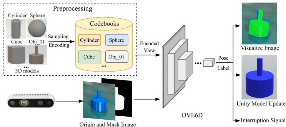
Fig. 2 The workflow of the object detection
