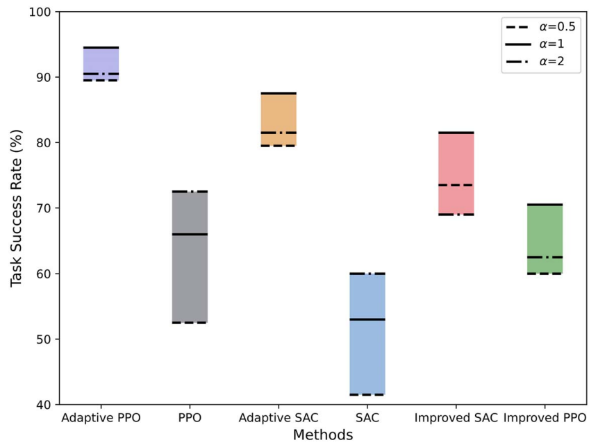
Fig. 11 Comparison of success rate for Pick and Place across different reward factors
