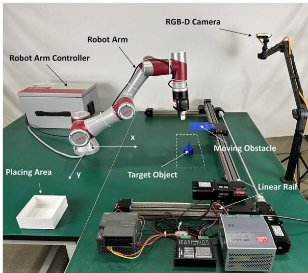
Fig. 6 Overall experiment setting
