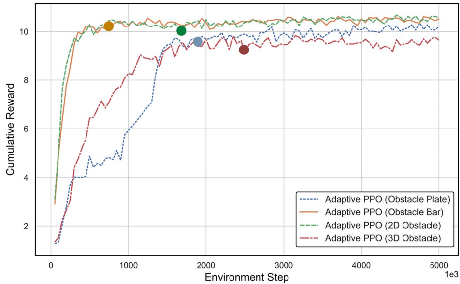
Fig. 13 Learning curve of the training process in obstacle plate, obstacle bar, 2D and 3D obstacle scenarios. The convergence step of each method is marked with circle dots.
