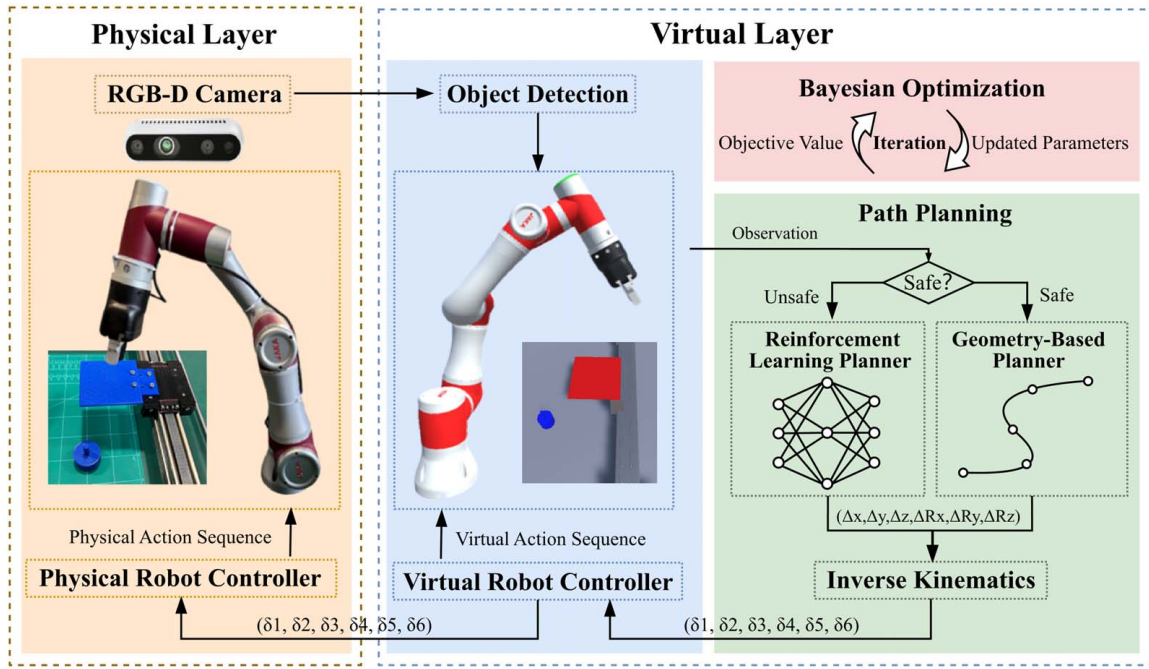
Fig. 1 Overall structure of the proposed adaptive robot motion planning approach
