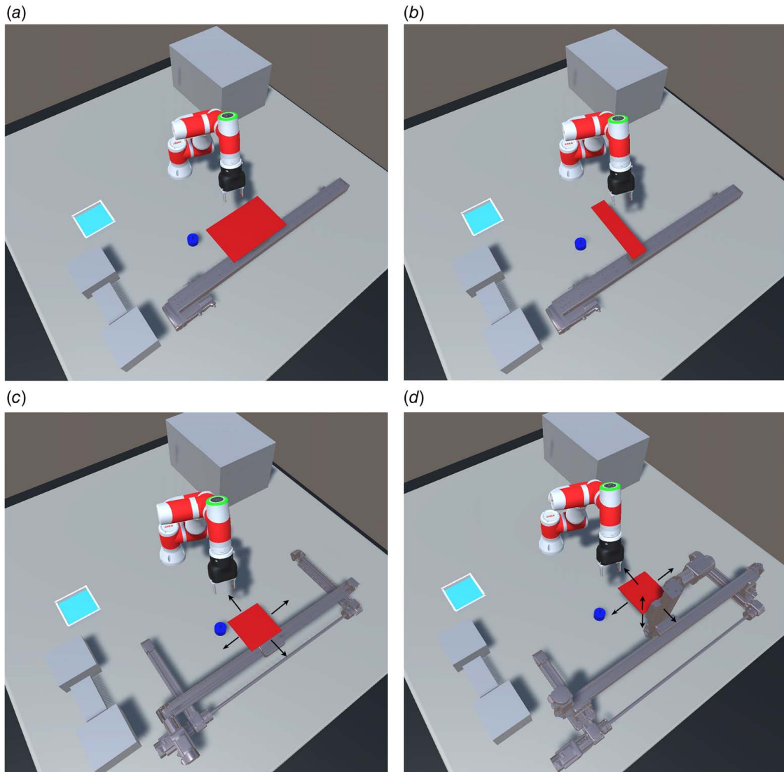
Fig. 12 Experiment settings on (a) obstacle plate, (b) obstacle bar, (c) 2D obstacle and (d) 3D obstacle
