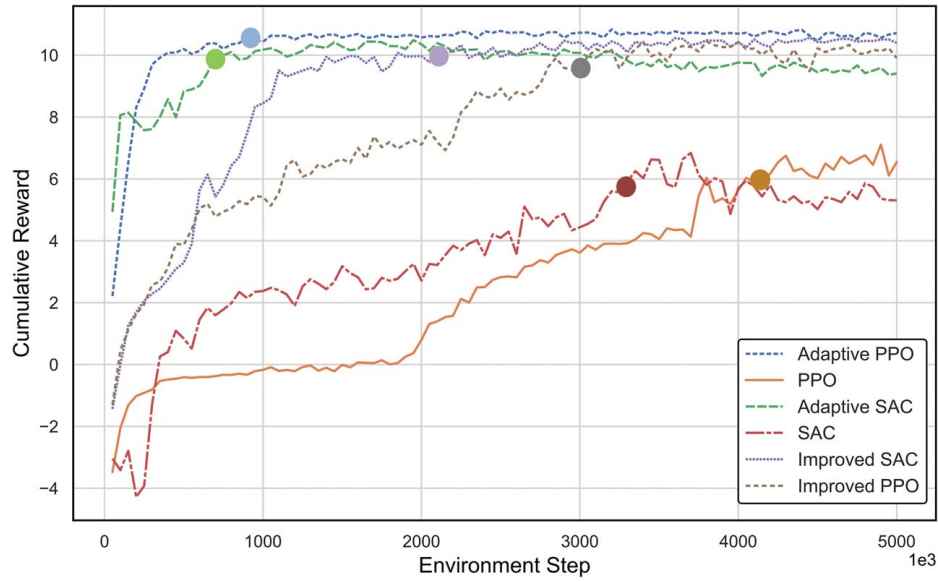
Fig. 9 Learning curve of the training process for different methods. The convergence step of each method is marked with circle dots.
