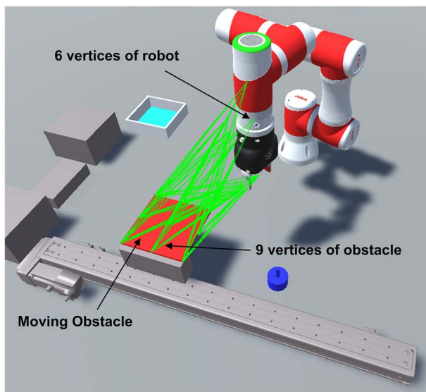
Fig. 4 Illustration of vertex-based distance detection. Here, six and nine vertices are selected from the robot and the surface of the obstacle, respectively. The lines between robot and obstacle indicate the detection lines between vertices.
