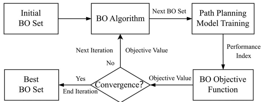
Fig. 5 Workflow of the Bayesian Optimization-based reward function parameter optimization method
