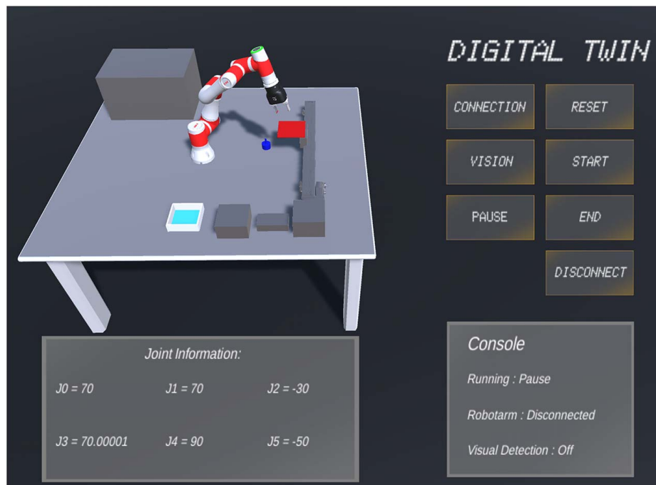
Fig. 7 The digital twin model of the robot and working environment with a user interface
