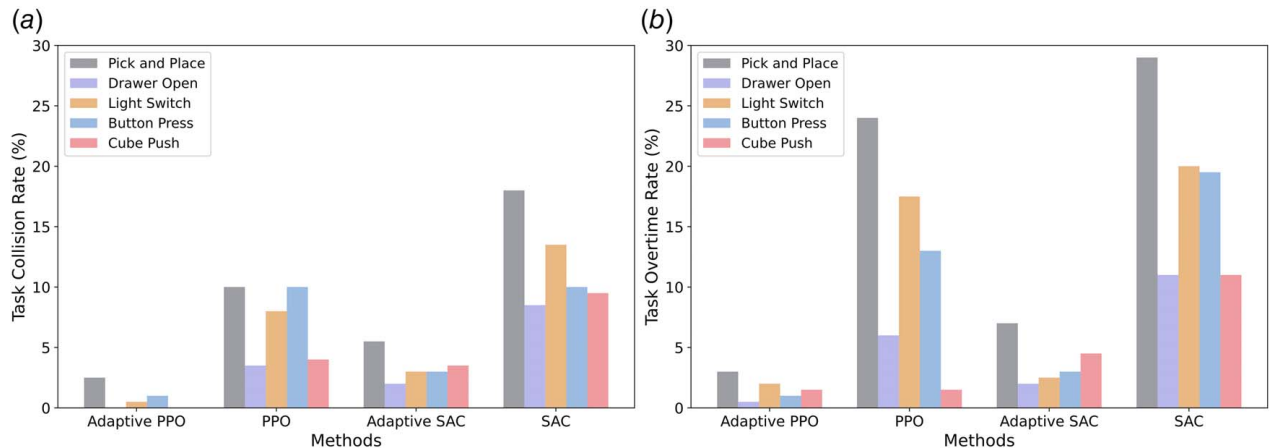
Fig. 10 Task performance comparison on (a) collision rate and overtime rate
